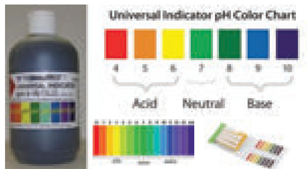
Figure 10.7 pH Indicator
