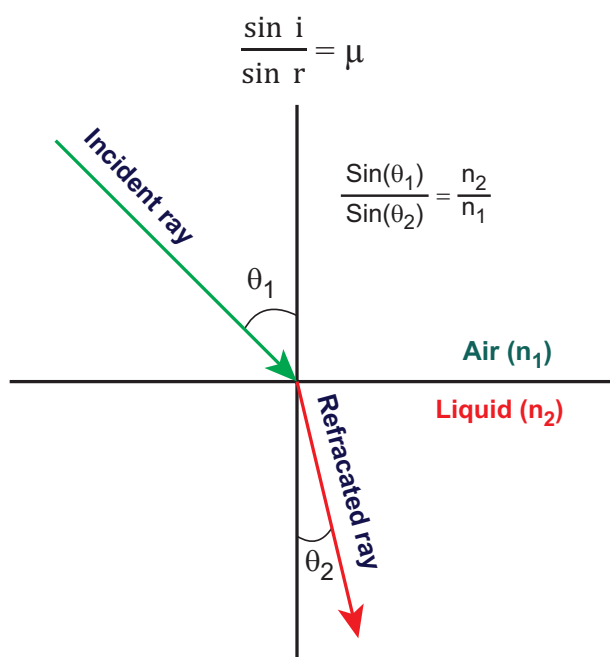
Figure 3.12 Snell's Law
