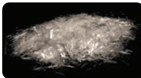
Figure 14.2 Benzoic acid crystals
