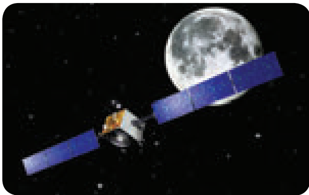
Figure 8.6 Chandrayaan - 1
