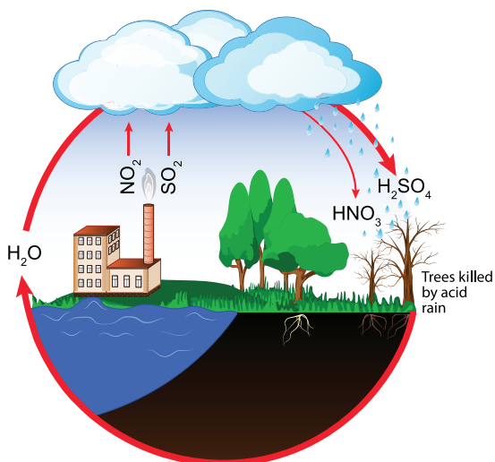
Figure 11.7 Acid rain
