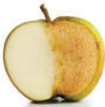
Fig 10.4 Browning of apple
