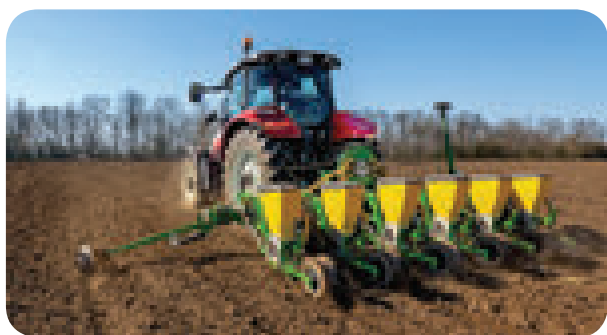
Figure 21.5 Seed Drill
