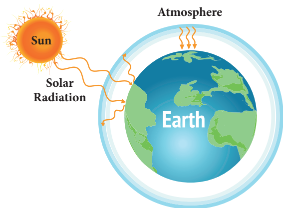
Figure 11.6 Greenhouse effect
