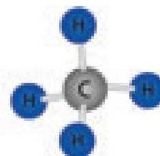
Figure 15.2 Structure of methane
