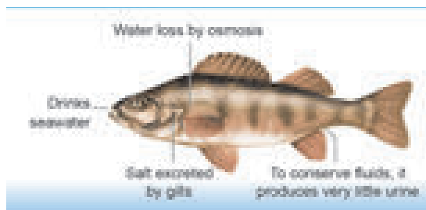
Figure 18.13 Osmoregulation by a marine fish
