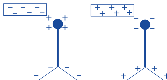
Figure 5.7 Movement of charges in electroscope near the top knob of the electroscope, the free electrons in the electroscope start to move up towards the knob. This means that the bottom has a net positive charge. The leaves will spread apart again now.
