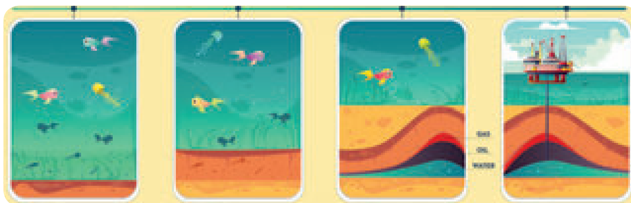
Figure 15.1 Formation of Hydrocarbons
