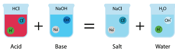
Figure 14.5 Acid – Base reaction
