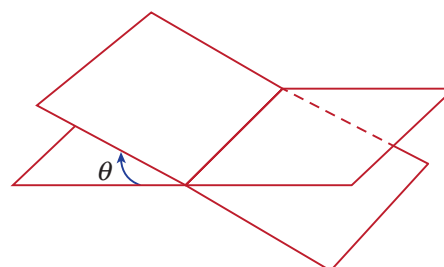
Figure 1.6 Plane angle
